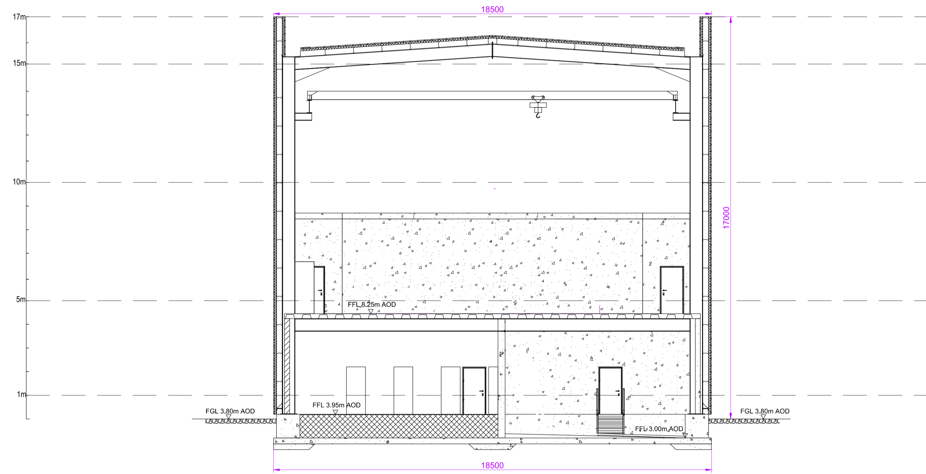
TRANSMISSION SUBSTATION - SECTION B-B
